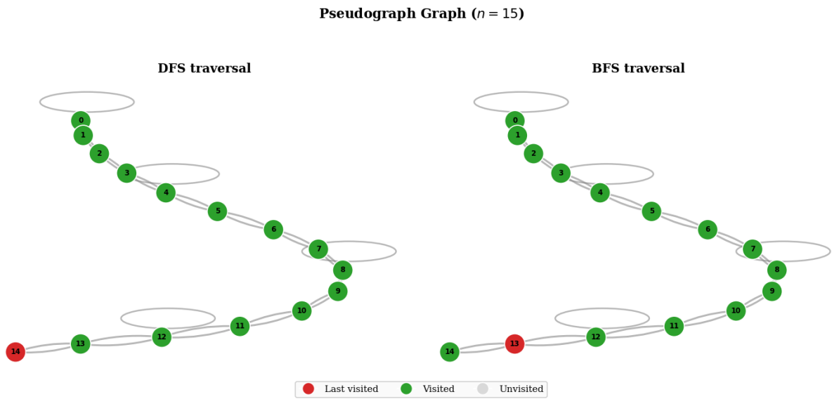
Figure 22: Pseudograph Traversal.
