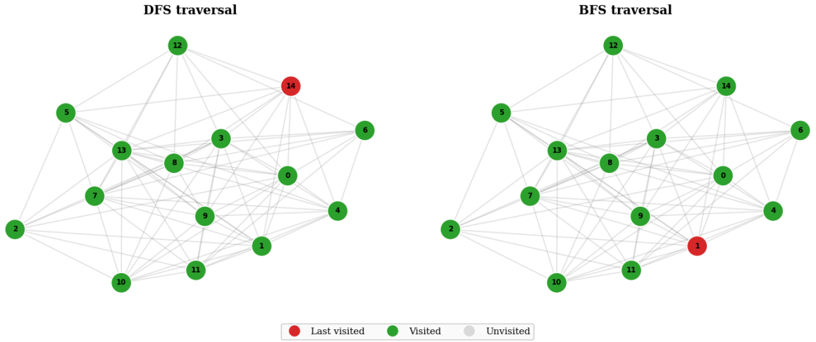
Figure 16: Dense Random Graph Traversal.
