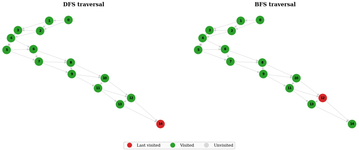
Figure 11: DAG Traversal.
