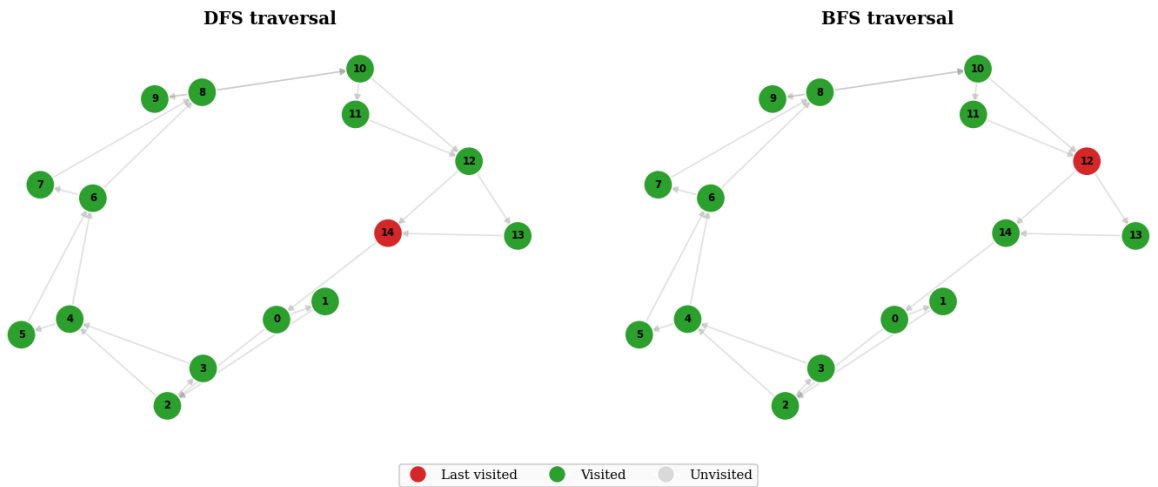
Figure 12: Directed Cycle Traversal.
